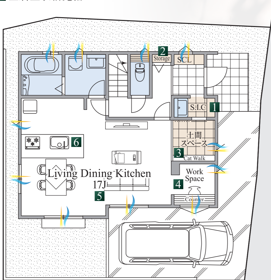
Floor1 52.99m 2
